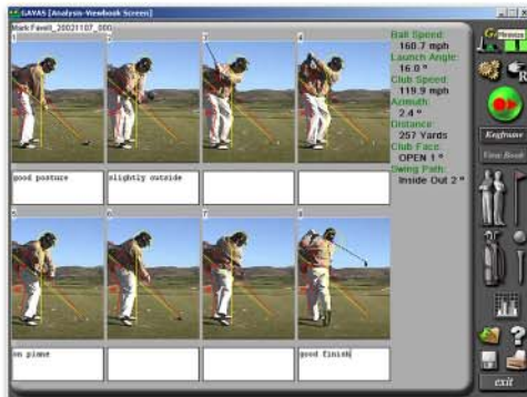
View-Book Screen
