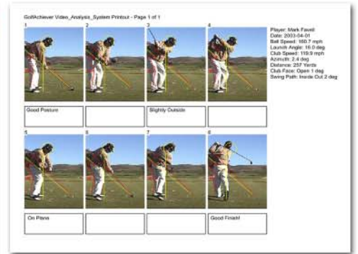
View-Book Printout
